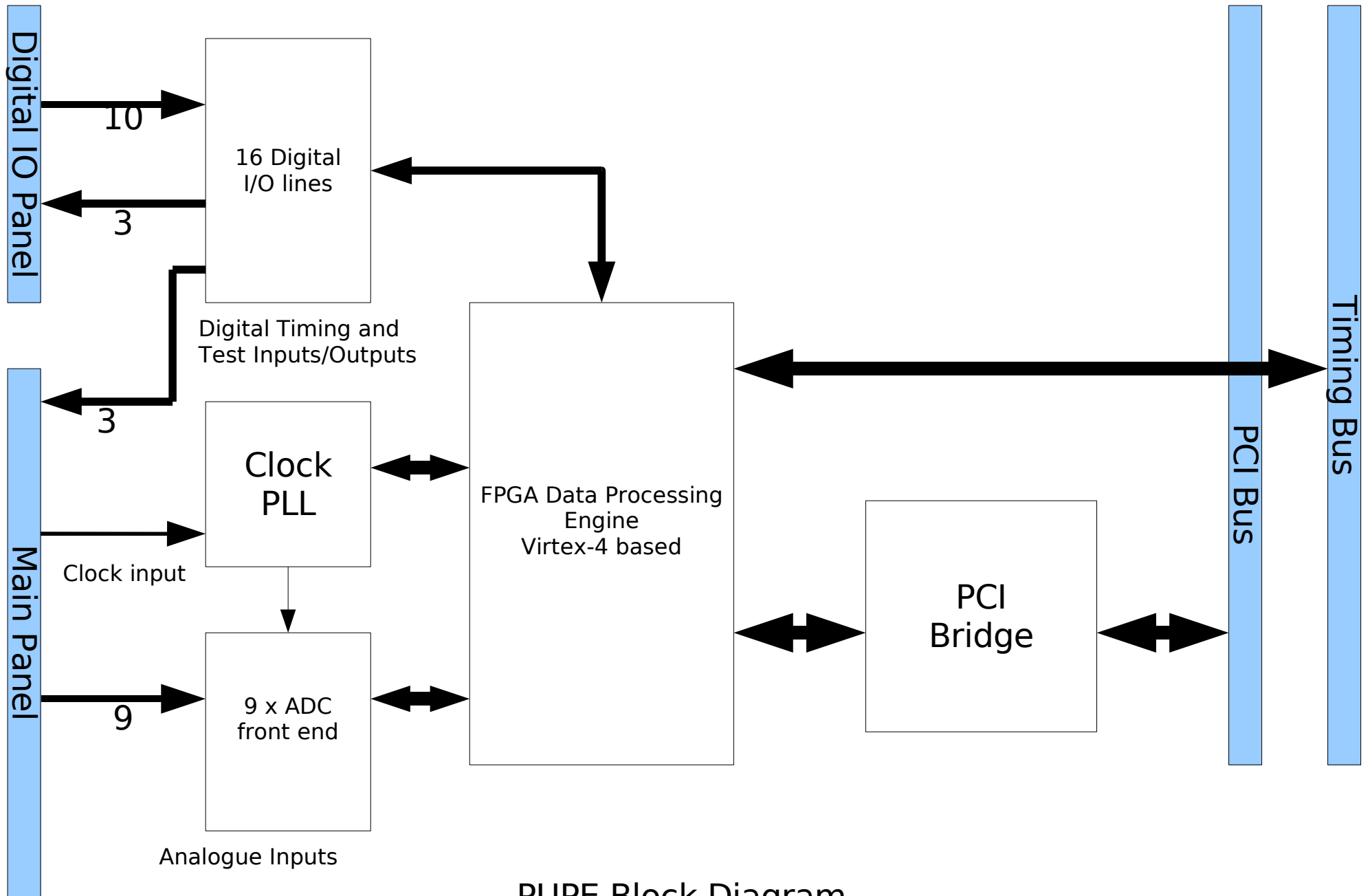
PUPE Block Diagram
